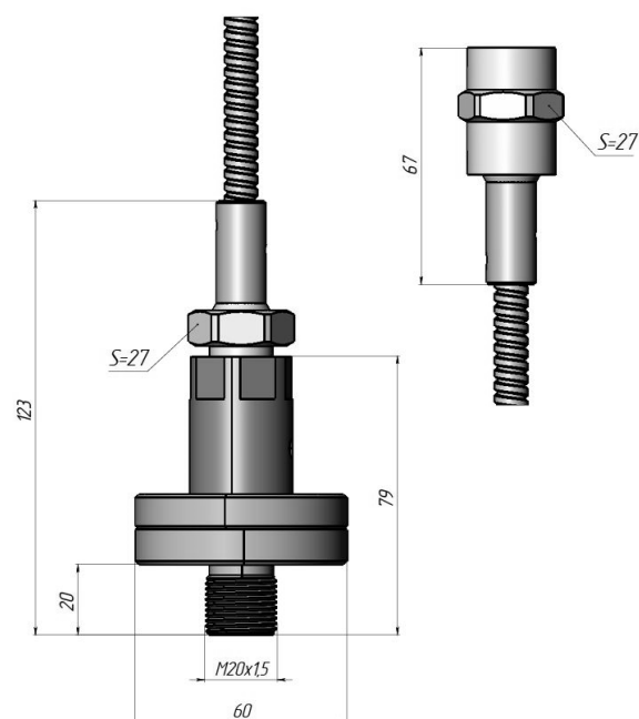
P-PP/K5-M20x1,5-316L/12X18H10T
