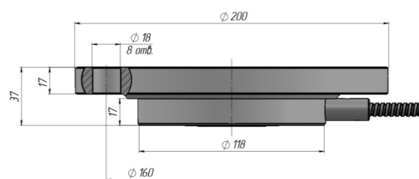
Φ-CP-DN80/PN16/E-316L/C-276
